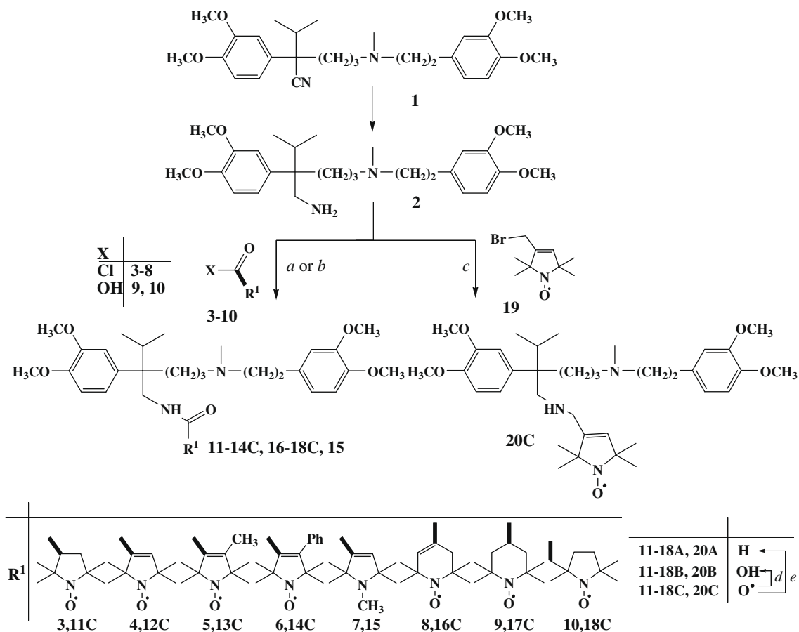
Scheme 1. Reagents and conditions: (a) 3–8 (1.1 equiv), Et 3 N (1.1 equiv), CH 2 Cl 2 0 °C→rt, 1 h; (b) 9, 10 DCC (1.0 equiv), 4-dimethylaminopyridin (0.05 equiv), rt, 24 h; (c) 19 (1.1 equiv), K 2 CO 3 (1.1 equiv), 18-crown-6 (cat.), CHCl 3 , reflux, 8 h; (d) EtOH/HCl, reflux, 20 min; (e) Fe (10 equiv), AcOH, 70 °C, 1 h, then K 2 CO 3 to pH 9.
