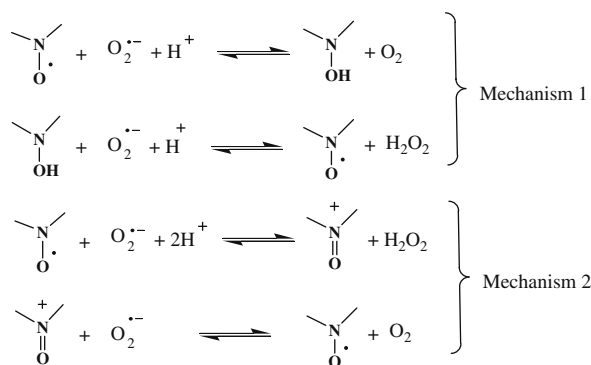
Figure 1. SOD mimetic mechanisms of cyclic nitroxides.
