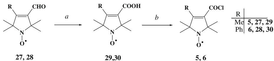
Scheme 3. Reagents and conditions: (a) \text{NaClO}_2 (1.1 equiv), \text{H}_2\text{O}_2 (0.9 equiv), \text{H}_2\text{O} –MeCN, \text{KH}_2\text{PO}_4 , 0 °C, 1 h, rt, then \text{Na}_2\text{S}_2\text{O}_5 , \text{H}^+ ; (b) \text{SOCl}_2 (1.23 equiv), pyridine (1.25 equiv), benzene, 0 °C, 10 min, then rt, 40 min.
