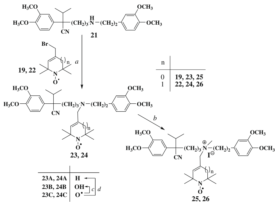
Scheme 2. Reagents and conditions: (a) 19 or 22 (1.1 equiv), K 2 CO 3 (1.1 equiv), 18-crown-6 (cat.), acetonitrile, reflux, 3–8 h; (b) 23 or 24 , MeI (5.0 equiv), 50 °C, 48 h; (c) EtOH/HCl, reflux, 20 min; (d) Fe (10 equiv), AcOH, 70 °C, 1 h, then K 2 CO 3 to pH 9.
